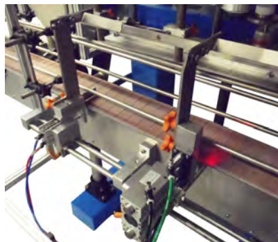
Turn Knobs for Adjusting Grippers
